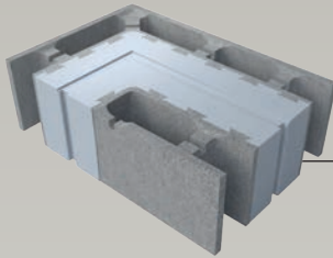
Thermal block 400 corner 600 x 400 x 200 mm 28 kg
