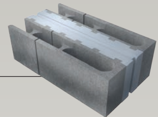
Thermal block 350 end 600 x 350 x 200 mm 30 kg
