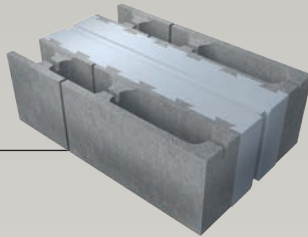
Thermal block 400 end 600 x 400 x 200 mm 27 kg
